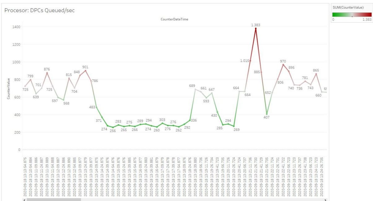
Slika 26: DPCs Queued/sec
