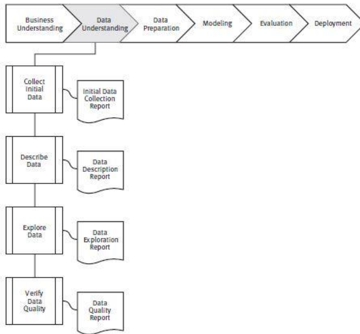
Figure 5: Data understanding
