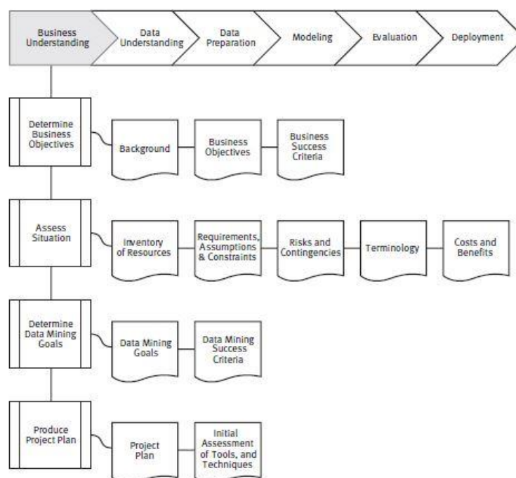
Figure 4: Business Understanding
