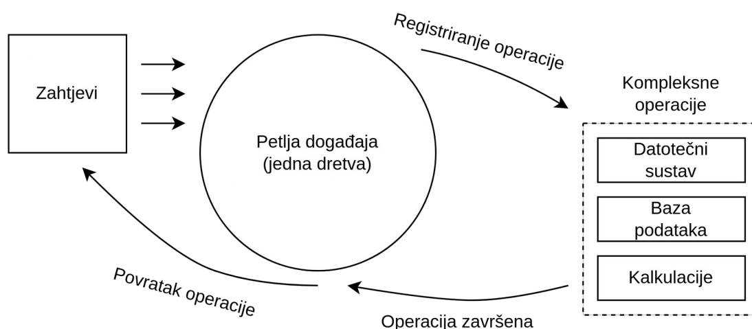
Slika 1: Prikaz rada Node.js (izvor: https://codeburst.io/the-only-nodejs-introduction-youll-ever-need-d969a47ef219 )
