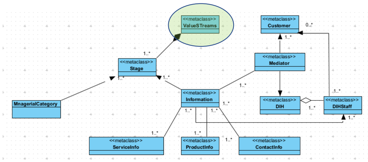
Fig. 56. DIH Value Stream Metamodel.
