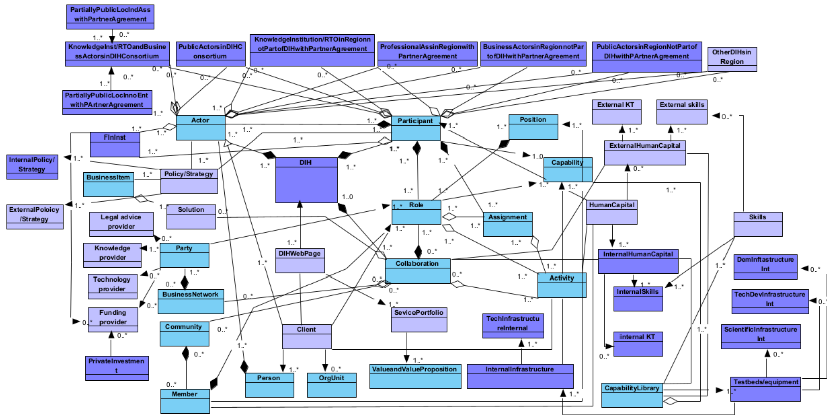
Fig. 88. Variant 4 of M1/1 DIH VDM (internal ecosystem).
