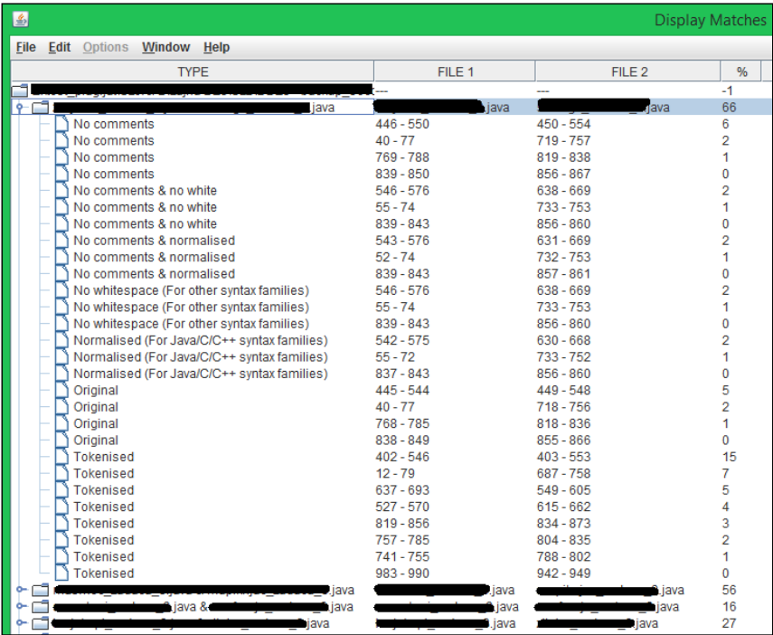
Fig. 6. Sherlock – Display matches.
