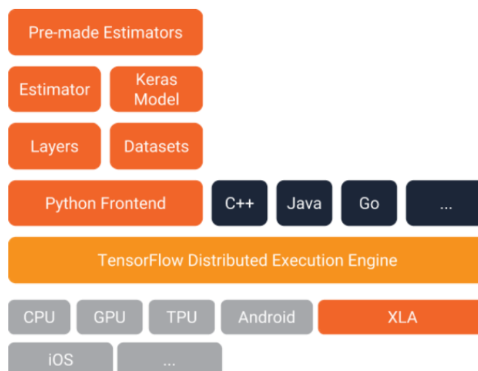
Figure 7 TensorFlow architecture [19]
