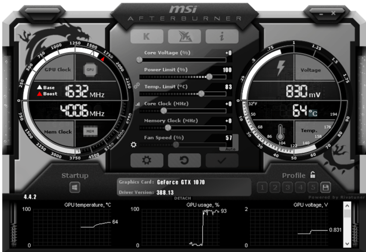
Slika 21: MSI Afterburner [35]
