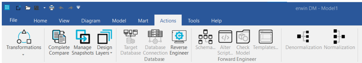
Slika 3.32 Erwin Actions
