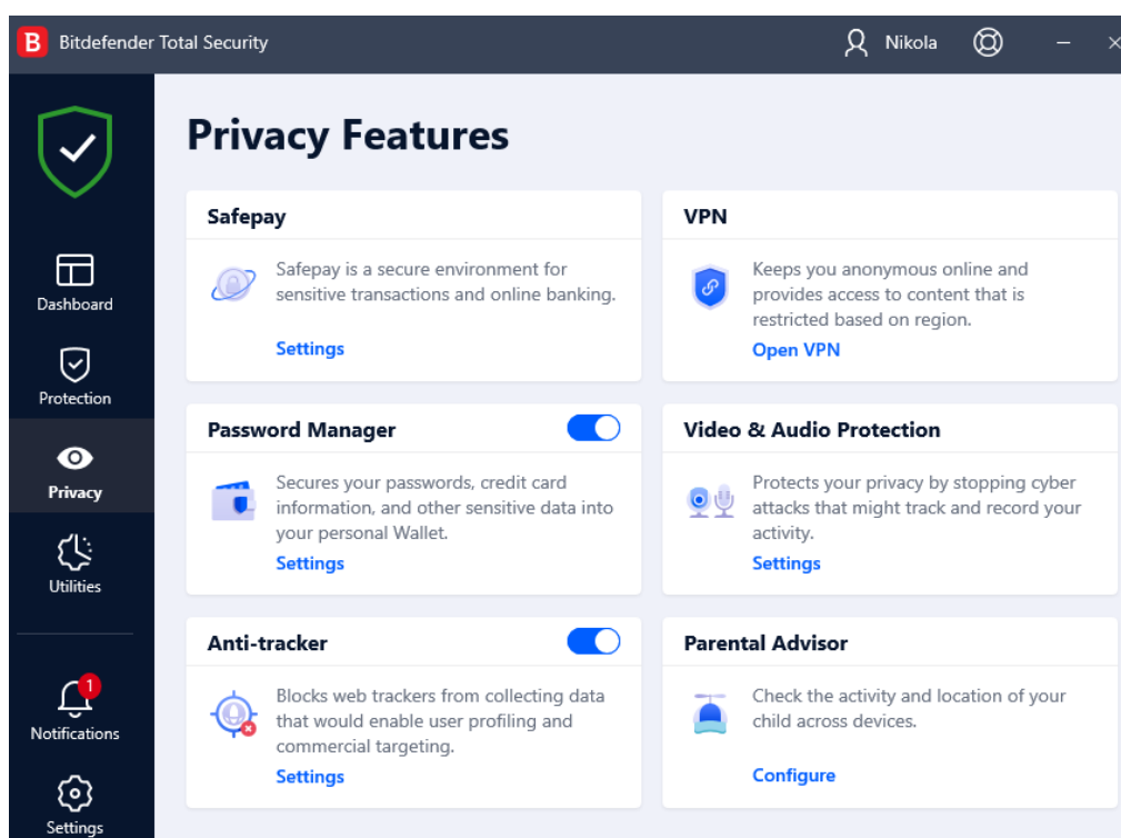
Slika 18: Bitdefender - Privacy
