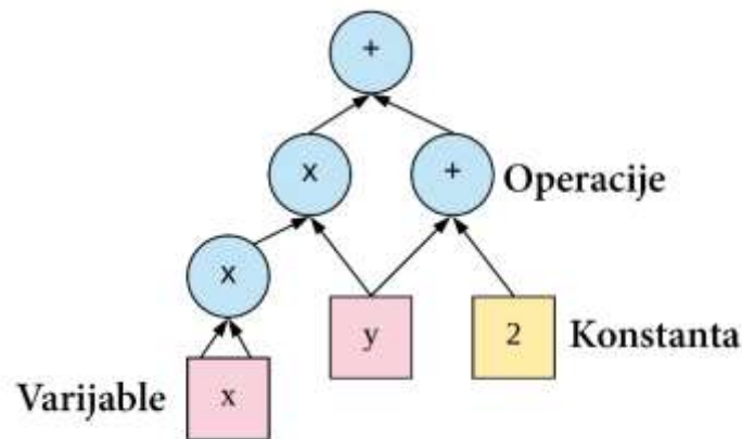
Slika 16: Shema računskog grafa u TensorFlowu (Easy-TensorFlow; 2018; izvor: https://www.easy-tensorflow.com/tf-tutorials/basics/graph-and-session )
