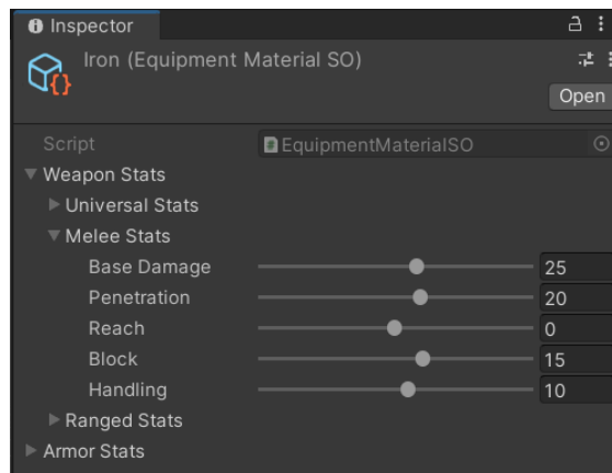
Slika 38. EquipmentMaterialSO, željezo (WeaponStats)
