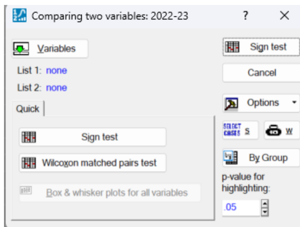
Slika 39: Prozor Comparing to dependent samples (variables) u Statistici (samostalna izrada)
